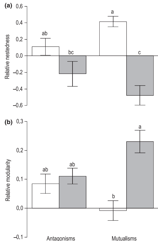
Figure 2 Analysis of the effect of interaction type and intimacy on relative nestedness (a) and modularity (b) of empirical bipartite networks. Columns depict the means and error bars depict standard errors. Grey columns depict sub-networks of intimate interactions, whereas white columns describe non-intimate interactions. Columns not sharing the same lower case letters are significantly different according to Tukey–Kramer tests .
